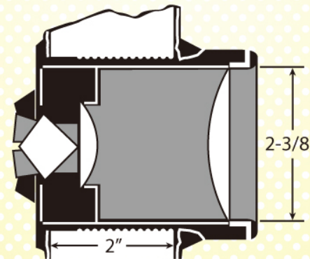
ADJUSTABLE FROM 1-1/8" TO 2"
